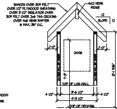
SECTION @ GABLE DORMER
