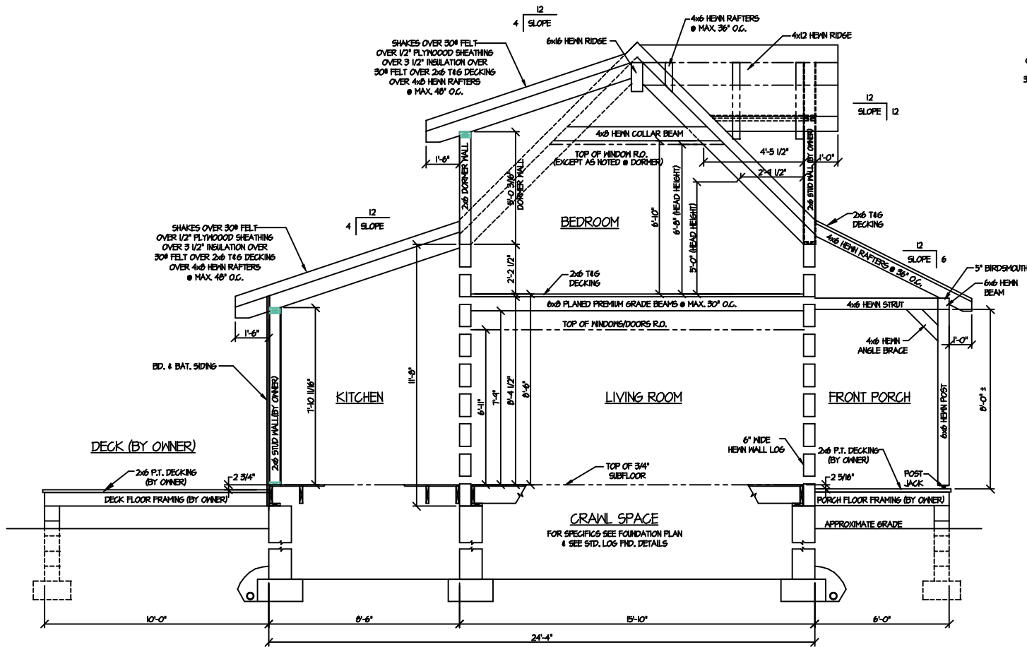
SECTION @ MAIN CABIN
