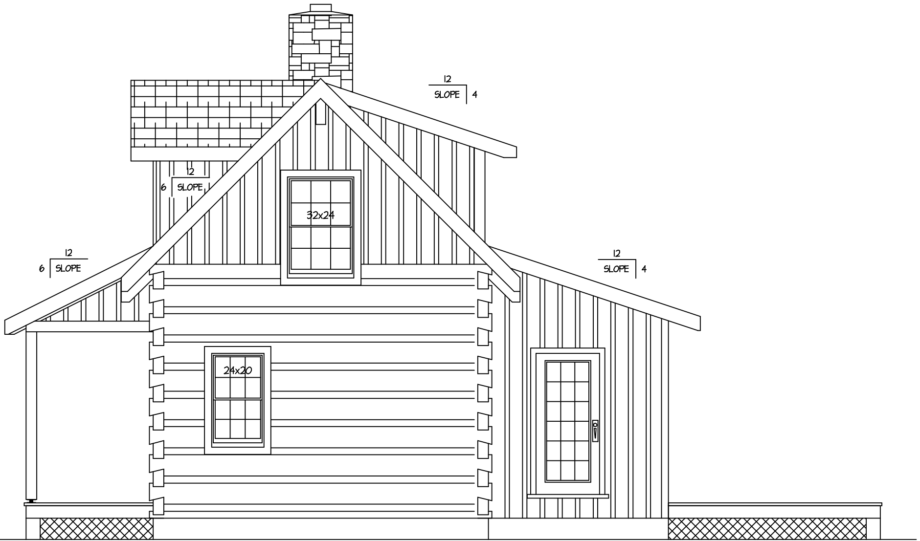
PLAN RIGHT
