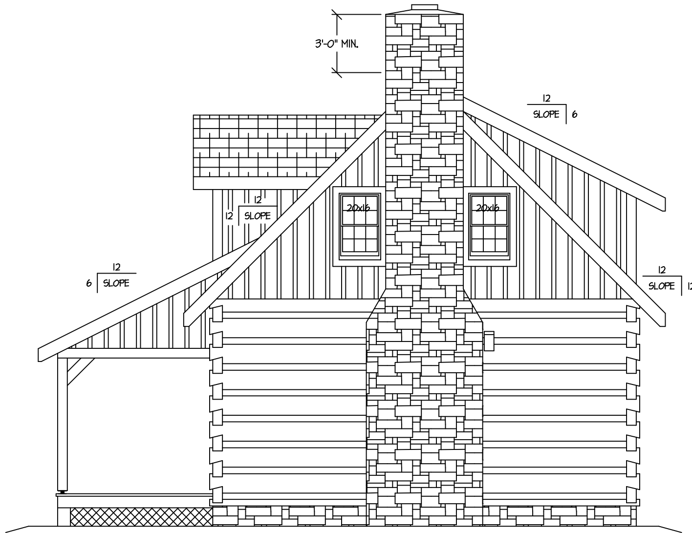
PLAN RIGHT
