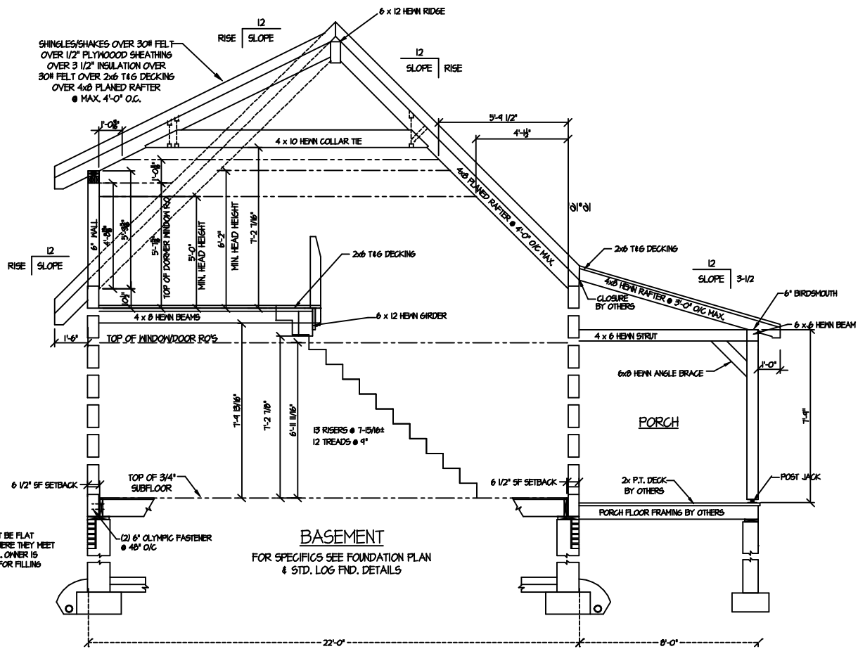
SECTION @ DINING/LIVING
