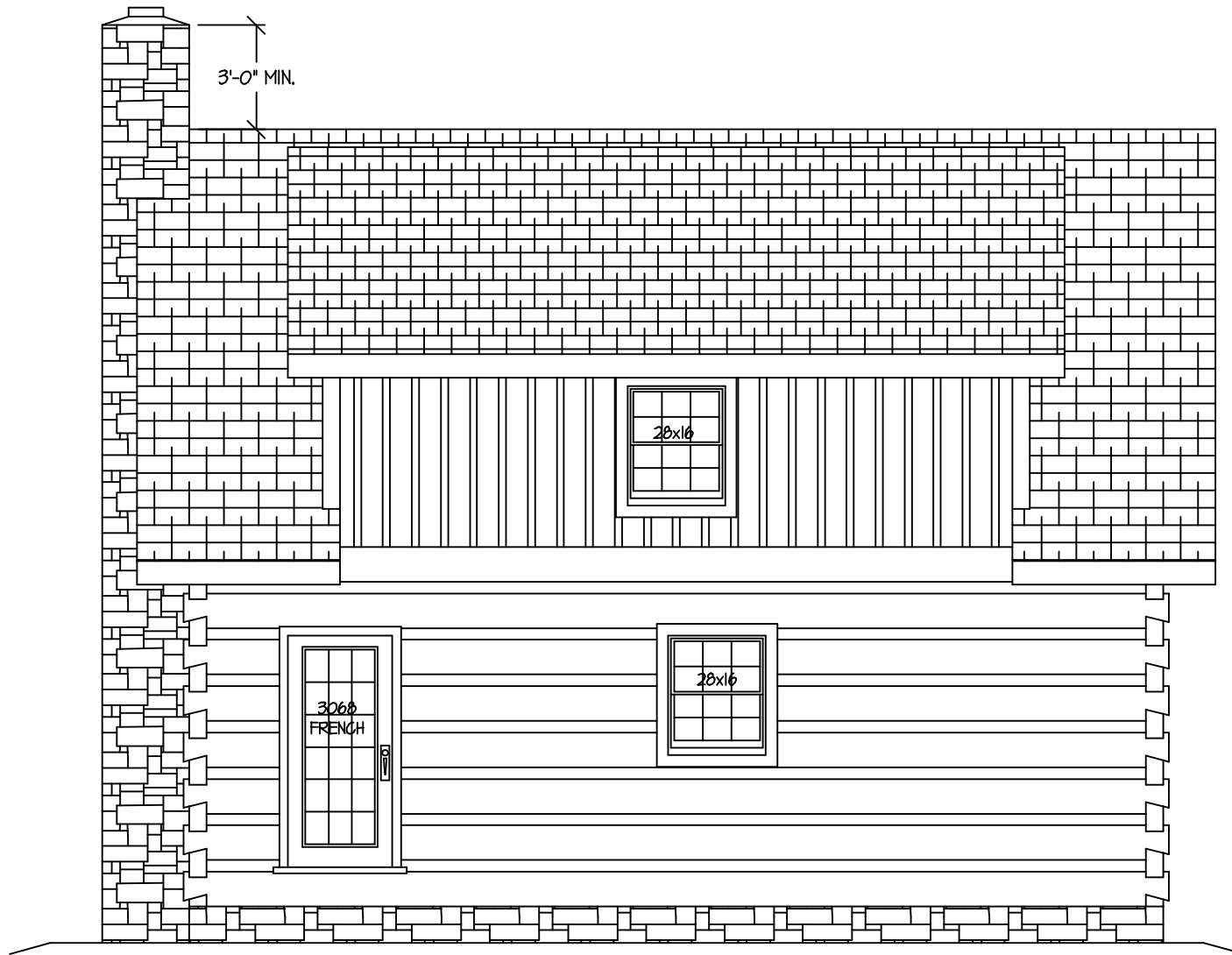
PLAN REAR
